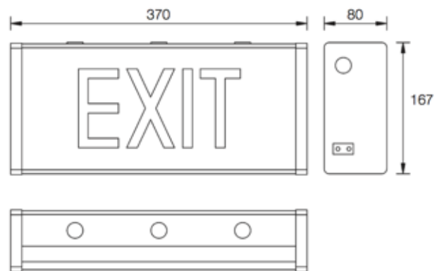
Dimension: mm NTS
