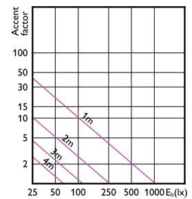
LEDspot MAS VLE 7-50W GU5.3 MR16 830 36D DIM
