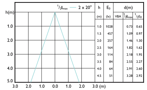
LEDspot MAS VLE 7-50W GU5.3 MR16 830 36D DIM
