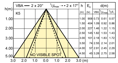
SDBE_LEDspotL_0109-Beam diagram
