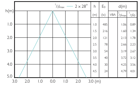
MAS VLE LEDspotLV 35W GU5-3 830 60D MR16
