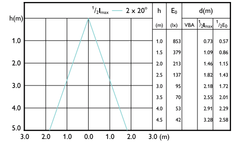
LEDSpot MR16 GU5.3
