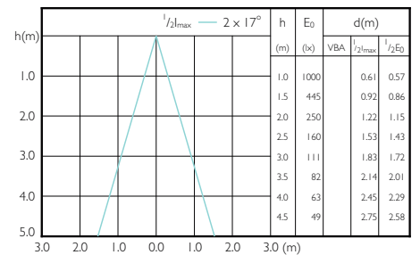
MAS VLE LEDspotLV 35W GU5-3 830 36D MR16
