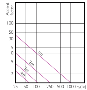
MAS VLE LEDspotLV 35W GU5-3 830 36D MR16
