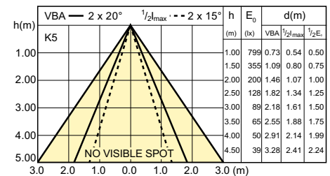
SDBE_LEDspotL_0115-Beam diagram
