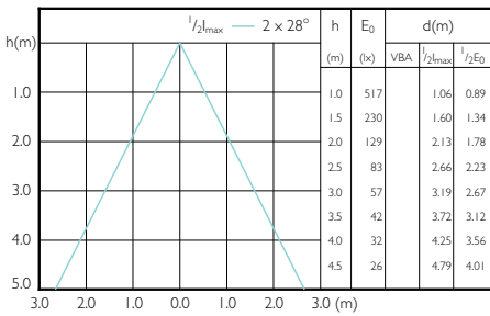
MAS VLE LEDspotLV 35W GU5-3 840 60D MR16
