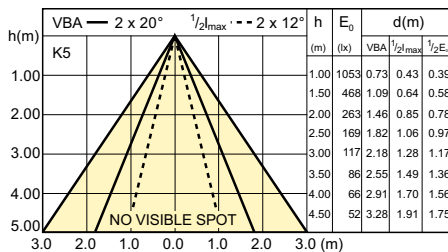
SDBE_LEDspotL_0113-Beam diagram
