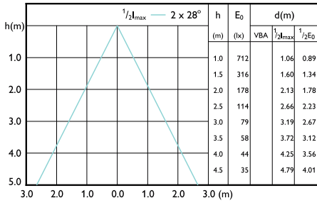
LEDspot MAS VLE 7-50W GU5.3 MR16 840 60D DIM
