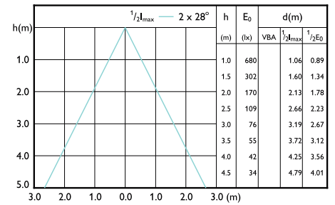
LEDspot MAS VLE 7-50W GU5.3 MR16 830 60D DIM
