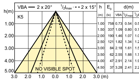
SDBE_LEDspotL_0114-Beam diagram
