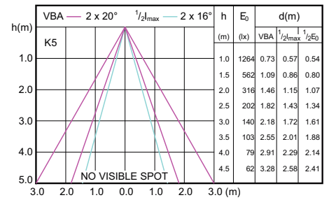
MASTER LED 5.5-50W MR16 GU5.3 4000K 450lm 36D
